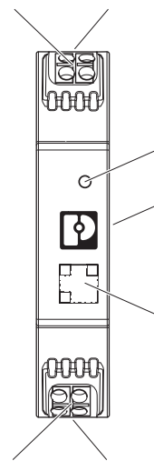
Figure 3 Location of functional elements and device connections
