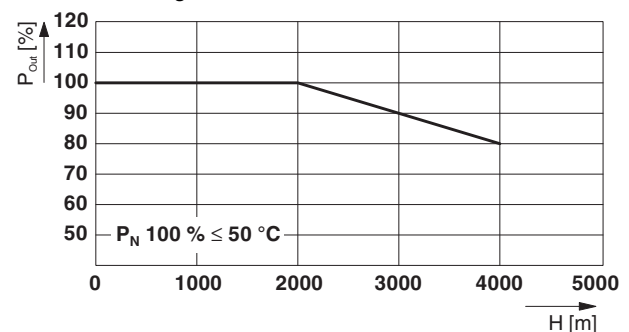
Figure 25 Output power depending on the installation height
