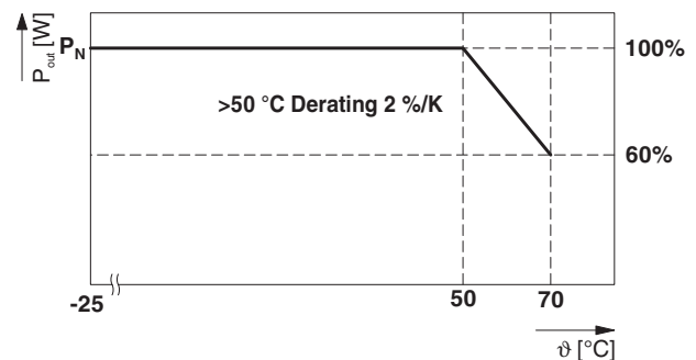
Figure 24 Output power depending on the ambient temperature
