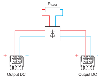
Figure 23 Schematic diagram, 1+1 redundancy with redundancy module (active or passive)
