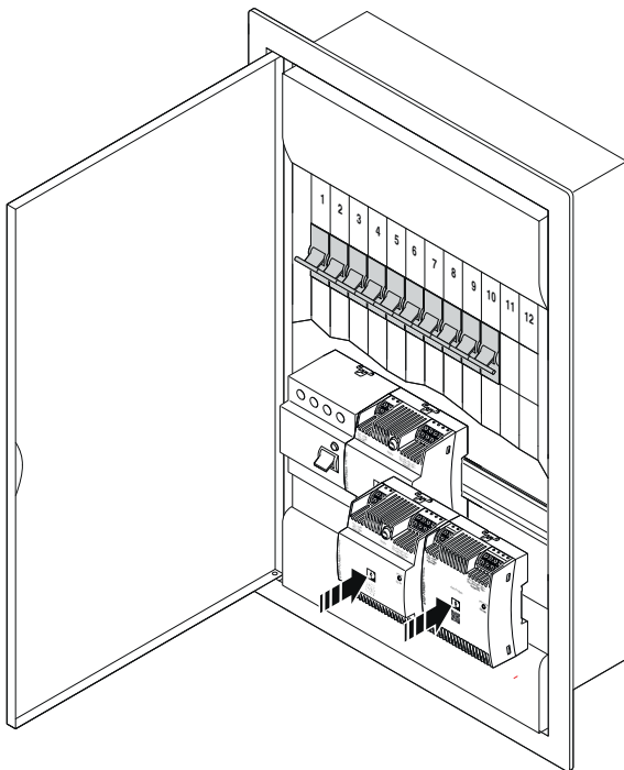
Figure 26 Schematic diagram, STEP POWER (4 HP) in a flush-mounted distributor (12 HP)
