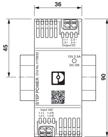
Figure 6 Device dimensions (dimensions in mm)
