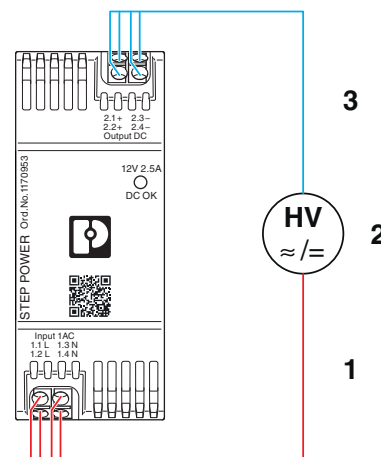
Figure 1 Potential-related wiring for the high-voltage test
