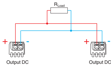
Figure 22 Schematic diagram, power increase in parallel operation
