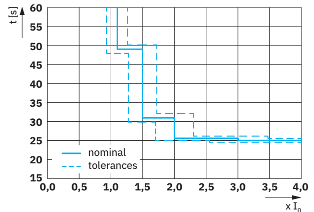
Figure 7 Tripping characteristics in HICCUP MODE
