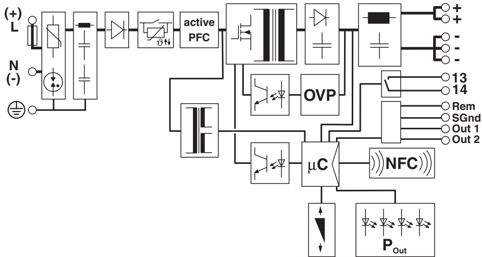
Figure 7 Block diagram
