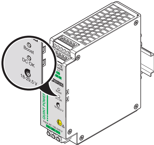
Figure 10 Signal outputs
