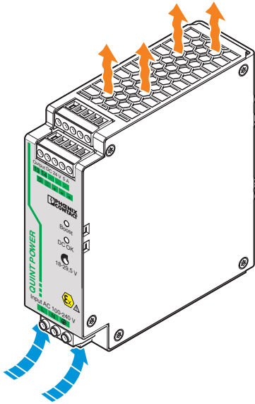
Figure 2 Convection
