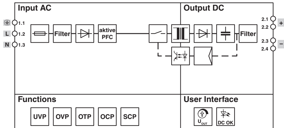
Figure 4 Block diagram
