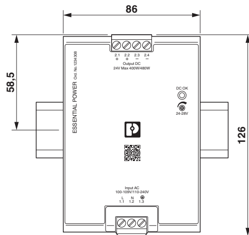
Figure 6 Device dimensions (dimensions in mm)
