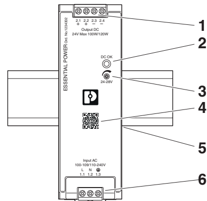
Figure 3 Location of functional elements and device connections
