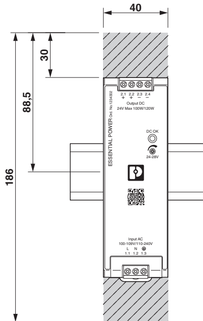
Figure 9 Device dimensions and minimum keep-out areas (in mm)
