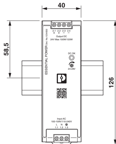
Figure 6 Device dimensions (dimensions in mm)
