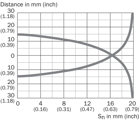
Response diagram
