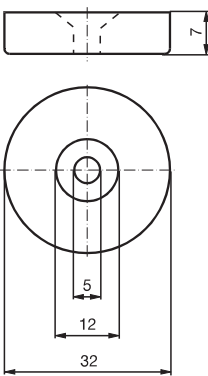
Magnet DM 25-32-07
