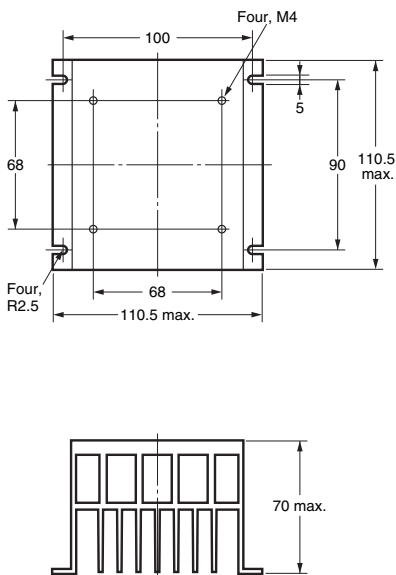
Mounting Holes
