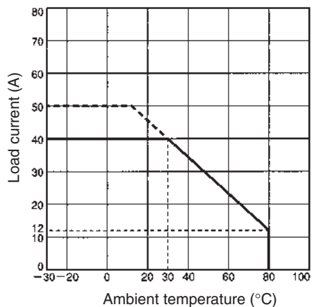
G3PA-450B-VD-2
