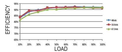
DDR-120C-48
