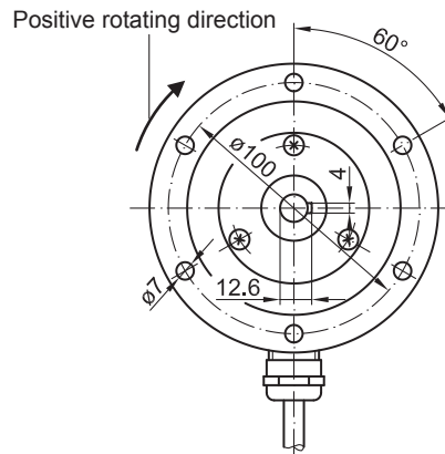
Version with connecting cable
