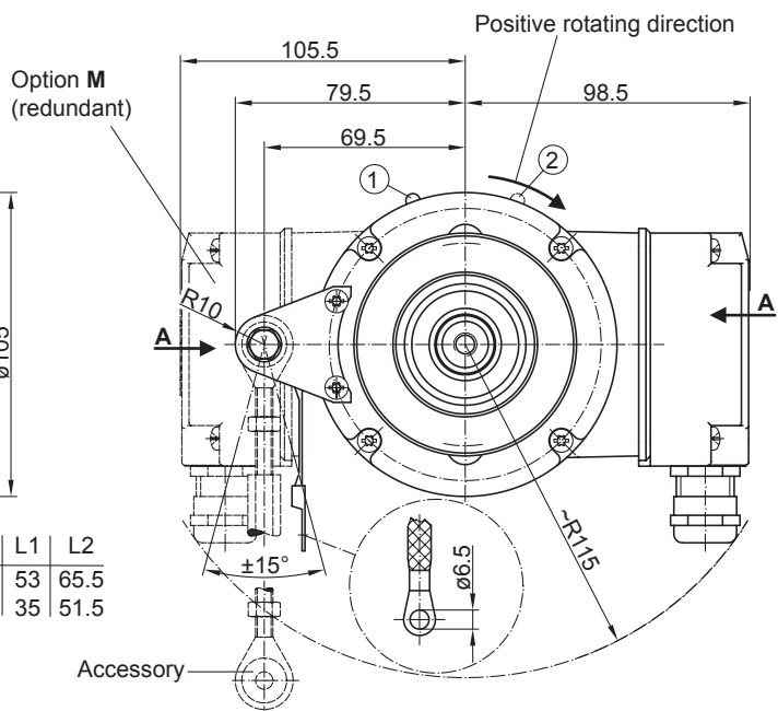
Blind hollow shaft
