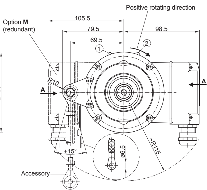
Cone shaft
