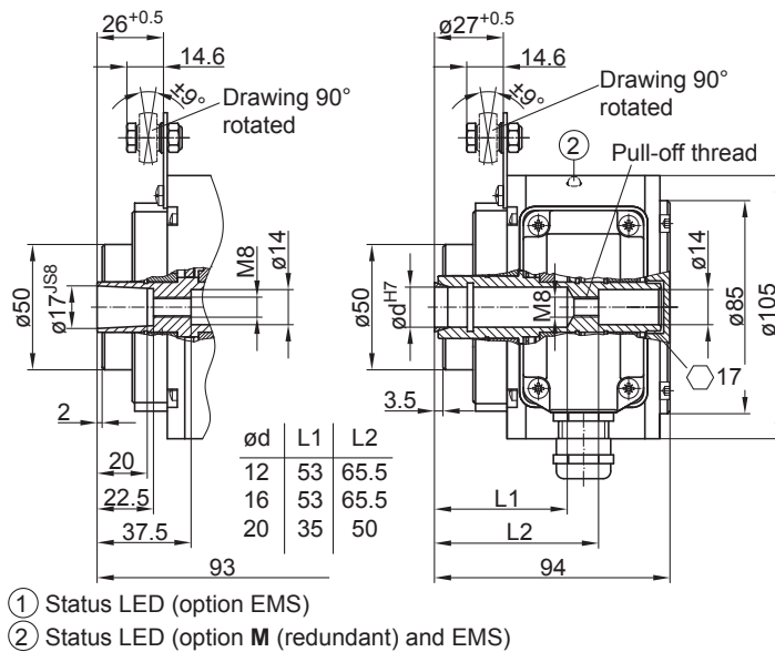
Version with radial terminal box
