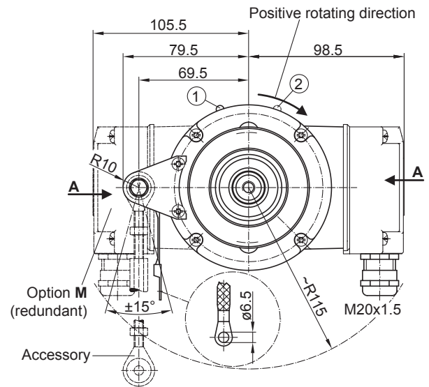
Version with radial terminal box
