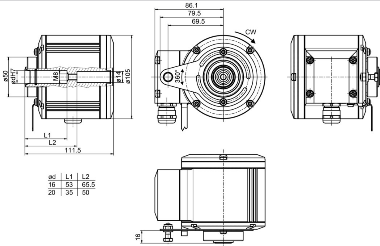
Blind hollow shaft with 1x terminal box (connection reference -P)
