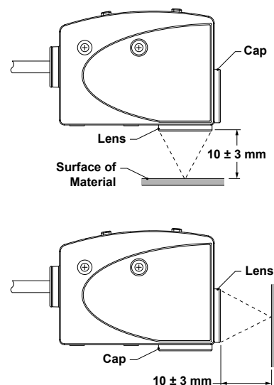
Figure 2. Mounting Distance and Lens Positions
