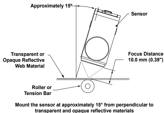
Figure 4. Mounting for Transparent and Opaque Material
