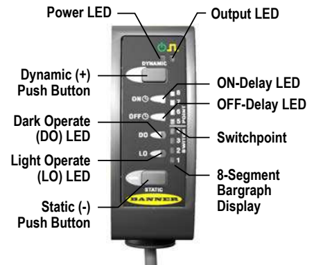
Figure 1. Sensor Features
